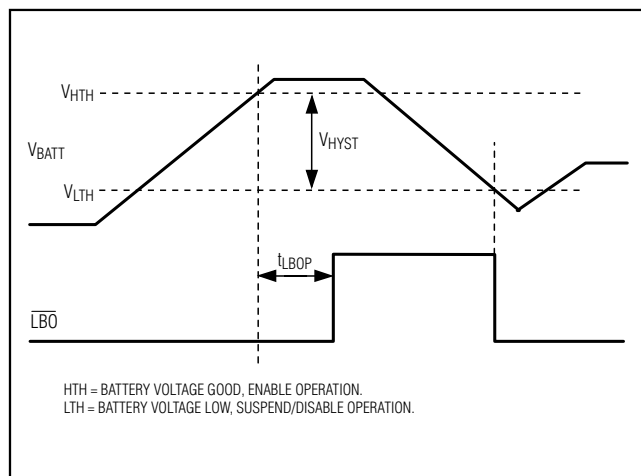
Figure 5. Hysteresis
